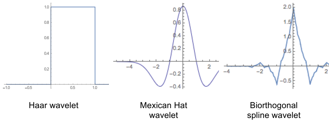
Figure 3. Examples of wavelets.
