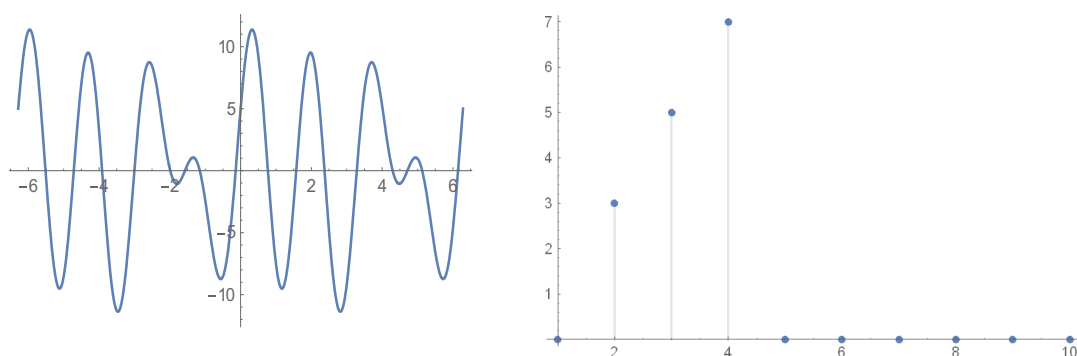
Figure 1. Function 3 \sin(2t) + 5 \cos(3t) + 7 \sin(4t) and its spectrum.
