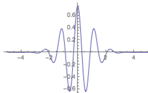
Figure 2. Example of Morlet wavelet.
